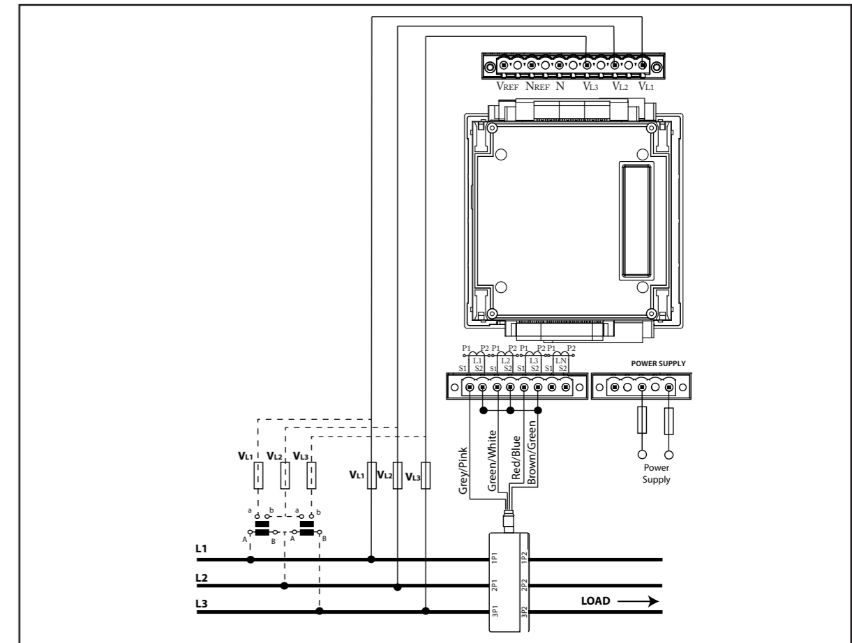
Red trifásica a 3 hilos / 3-wire three-phase network Transformadores de corriente serie MC3 (.../0.250 A) / MC3(.../0.250A) serial current transformers
