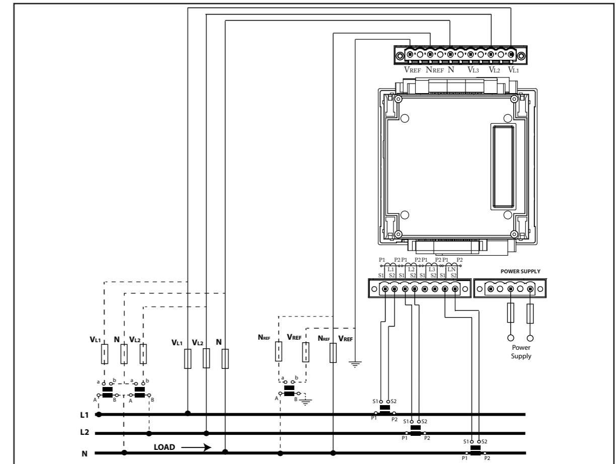
Red bifásica a 3 hilos / 3-wire two-phase network Transformadores de corriente .../5A o .../1A / .../5 or .../1A current transformers
