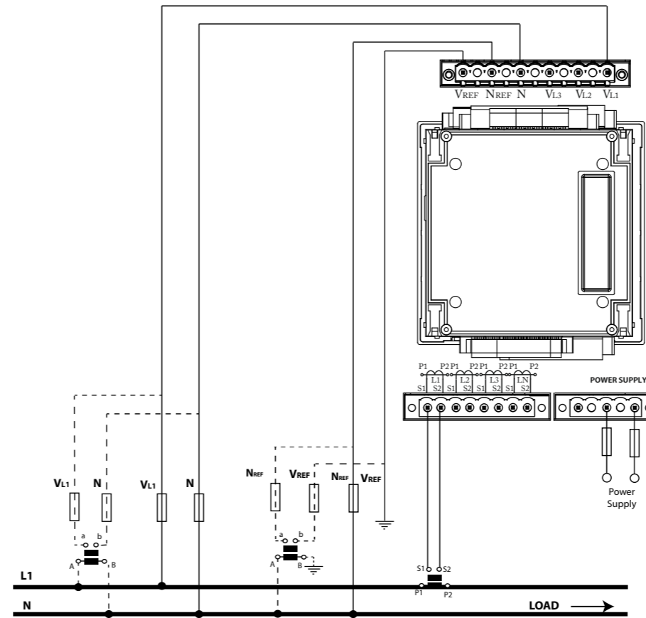
Red monofásica fase-neutro de 2 hilos / 2-wire Single-phase network (Neutral) Transformadores de corriente .../5A o .../1A o .../5 o .../1A current transformers
