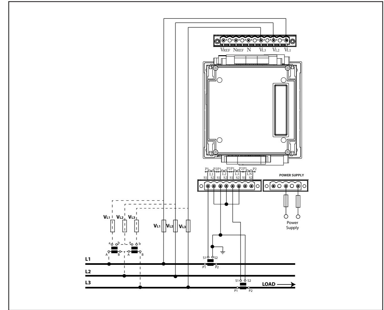
Red trifásica a 3 hilos / 3-wire three-phase network (ARON) Transformadores de corriente .../5A, o .../1A / .../5, or .../1A current transformers
