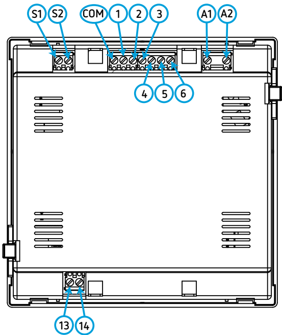
Figura 2: Bornes del computer C6 Wi-Fi
