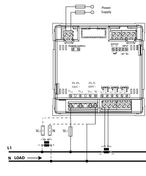
Red monofásica fase-neutro de 2 hilos 2-wire Single-phase network (Neutral)
