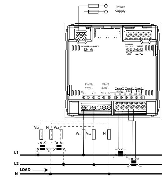
Red bifásica a 3 hilos / 3-wire two-phase network
